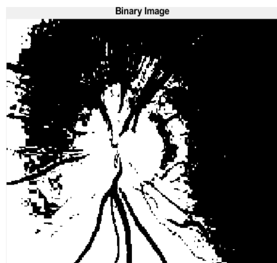
Figure 5.4 Binary image
