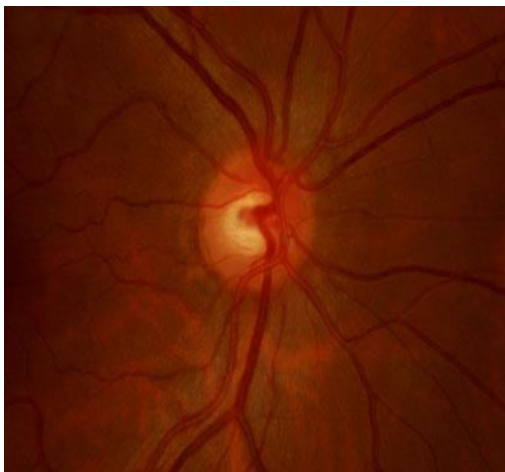
Figure 5.1: RGB Image
