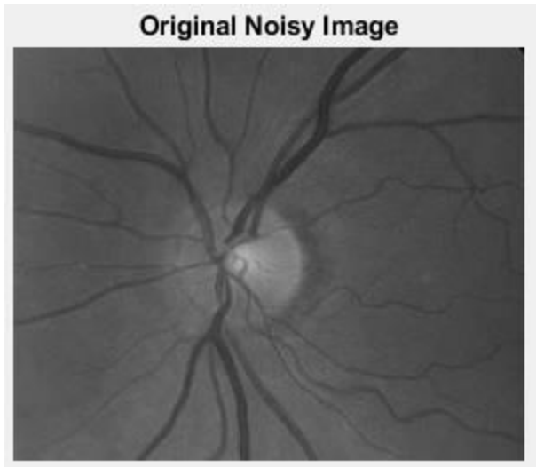
Figure 5.5: Noisy Image
